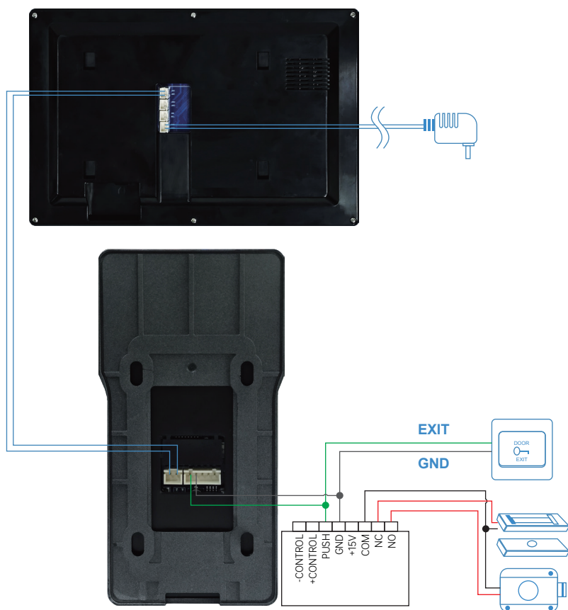
Access Control Power Connection Diagram
